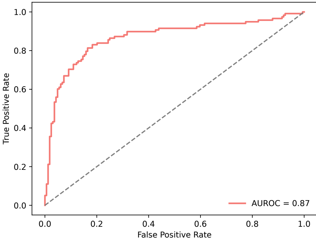
SVM ROC Curve
